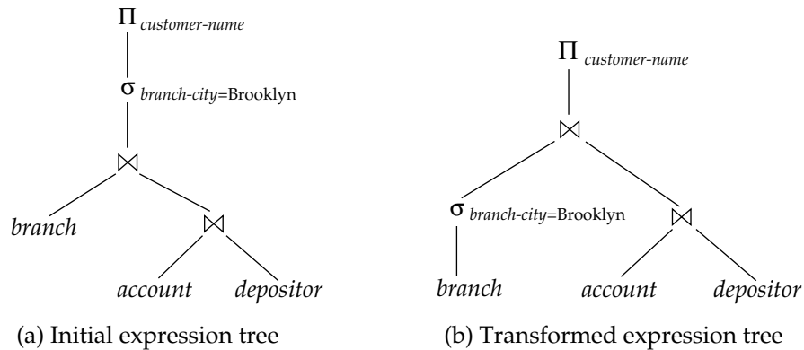
Figure 14.1 Equivalent expressions.
